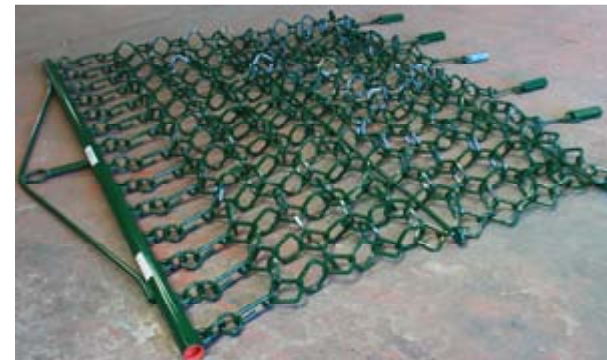
Series 09 Model 9132 2.44M (8') wide, 1.5M (5') Deep Mesh Chain Harrow shown
